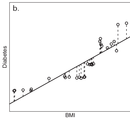
Figure 11 (a) The best-fit regression line for the model “Diabetes = -7.38431 + 0.55593 \text{ BMI} .” (b) The dashed vertical lines illustrate the residual for each instance.
